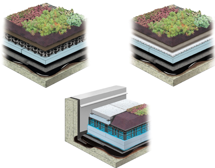
Typical stormwater management assemblies
