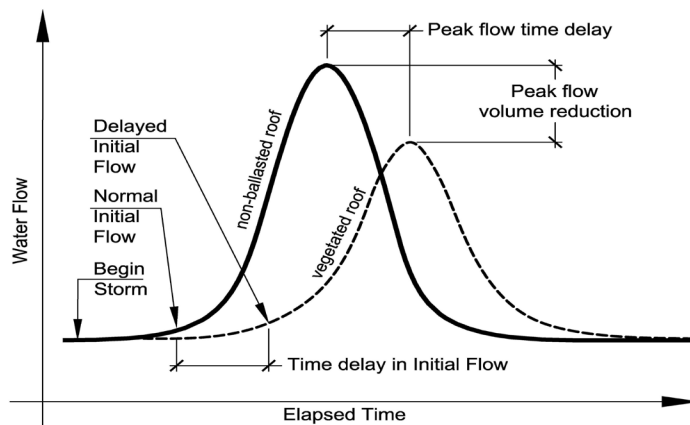
Stormwater hydrograph
